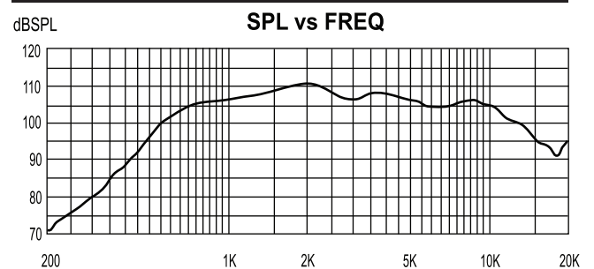
Response of horn with PreNeo-740N
