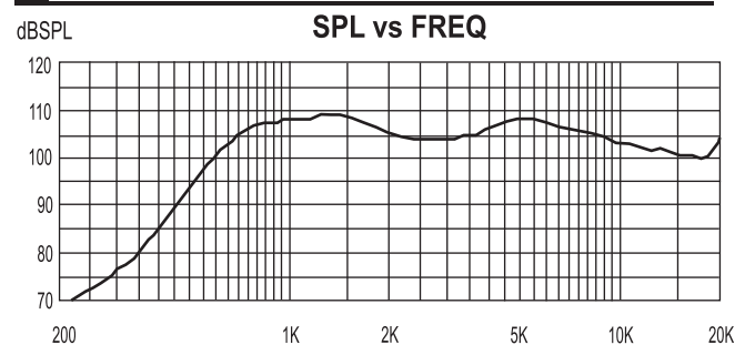
Response of horn with BM-D440S
