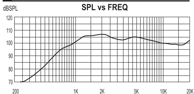
Response of horn with BM-D440S
